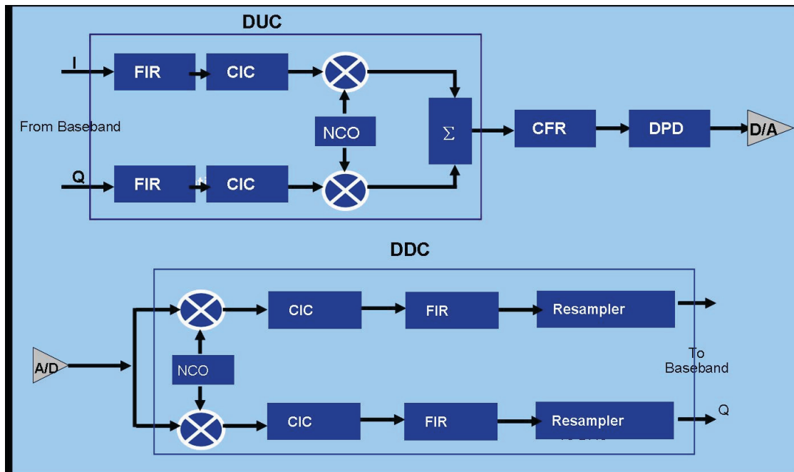
Figure 3. Digital IF Processing Functions
