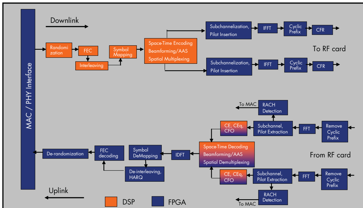
Figure 1. DSP/FPGA Partitioning for OFDMA Systems
