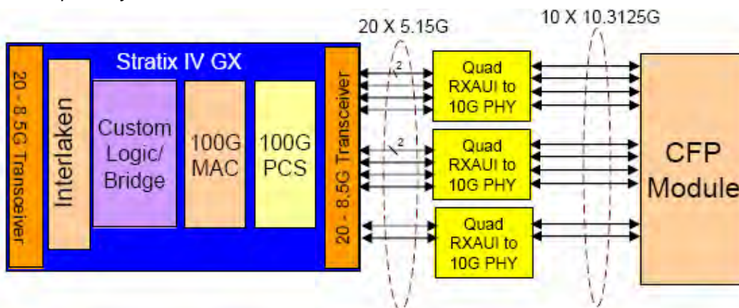
Figure 11. Complete System Solution
