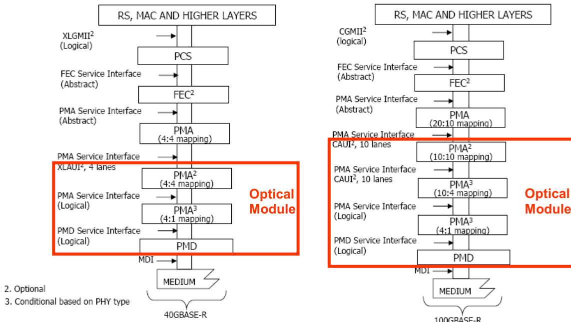
Figure 5. 40GbE/100GbE Interface
