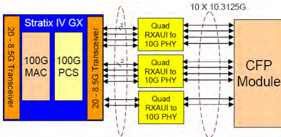
Figure 10. 100G MAC Solution
