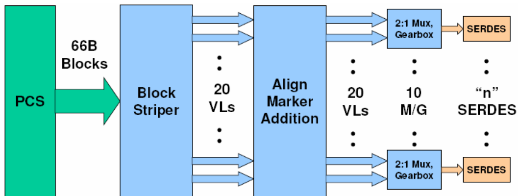
Figure 7. Transmit Path of the PCS Channel
