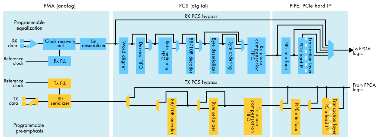
Figure 2. Stratix IV GX Transceiver Block
