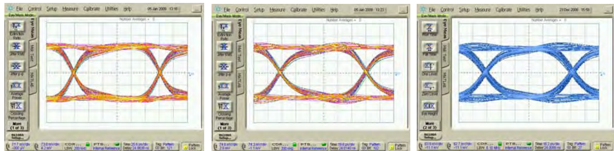
Figure 3. Transmitter "Eye" at 6.25 Gbps (left), 8.5 Gbps (center), and 10 Gbps (right)
